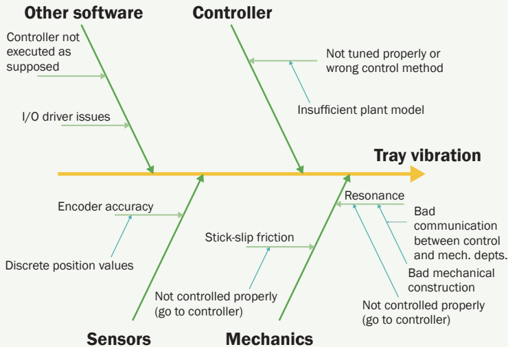
Figure 3.2. Ishikawa diagram for conveyor problem.
