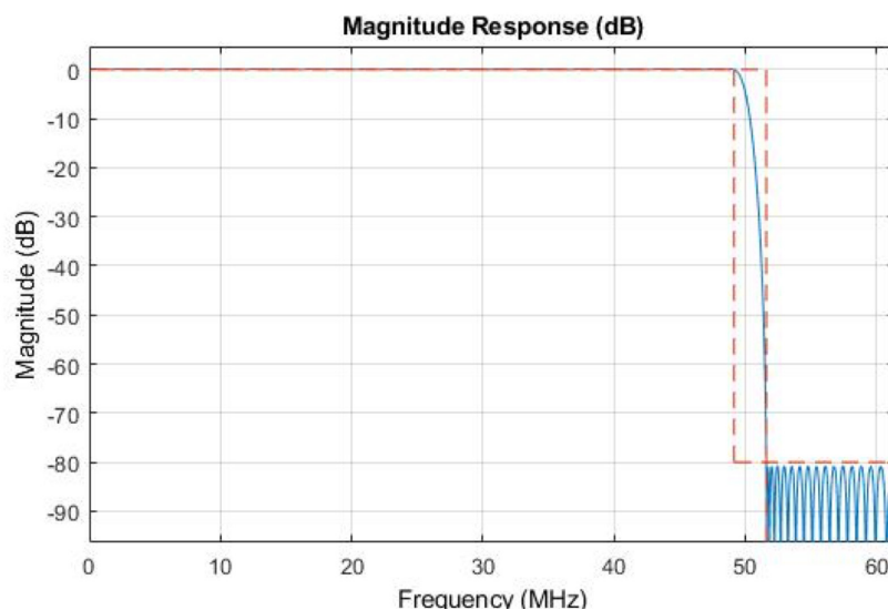
Figure 6. Magnitude of the filter response for the NR-FR1-TM3.1a waveform.
