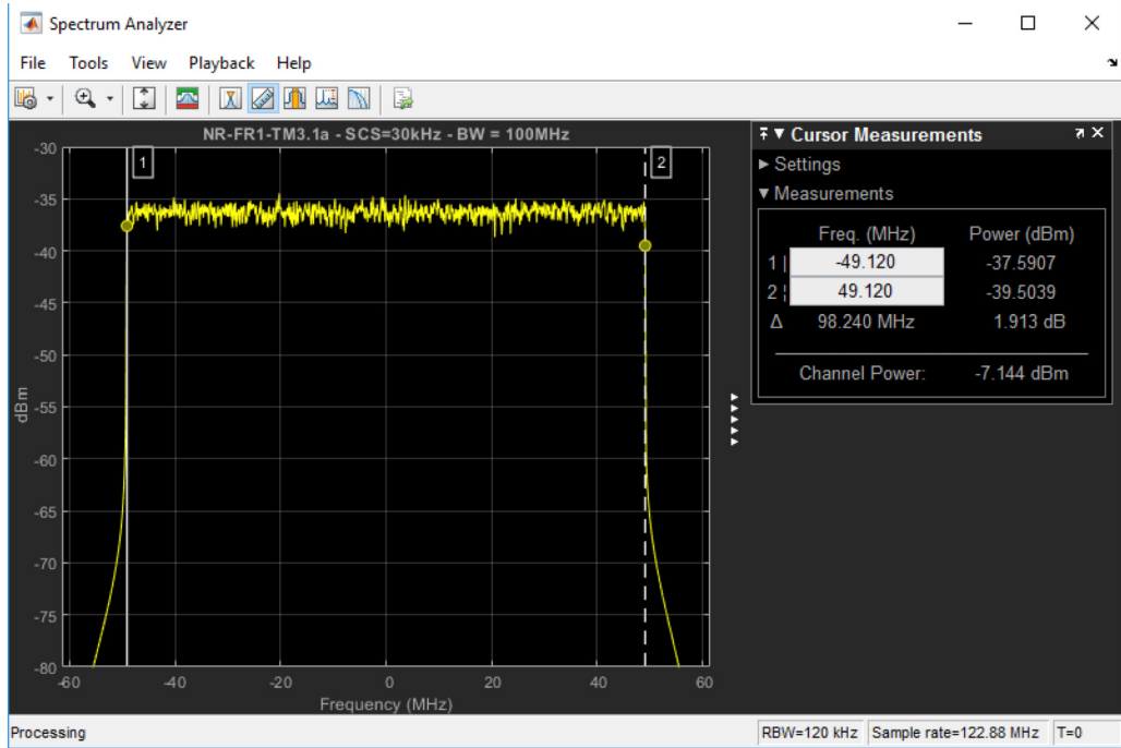
Figure 4. Spectrum of NR-FR1-TM3.1a waveform with 100 MHz bandwidth and 30 kHz subcarrier spacing.
