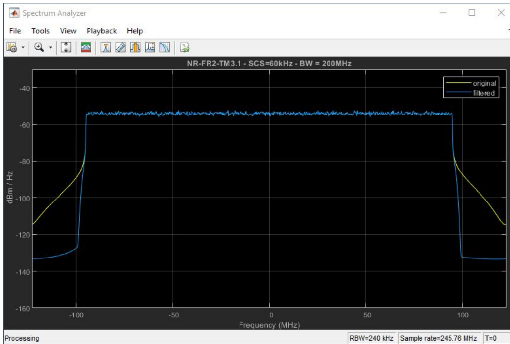
Figure 7. Spectrum of NR-FR1-TM3.1a waveform with and without filtering.
