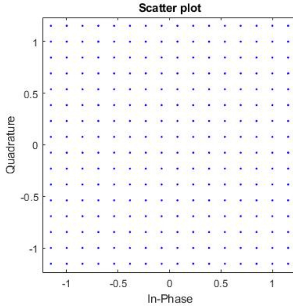
Figure 8. 256QAM constellation recovered in the receiver.
