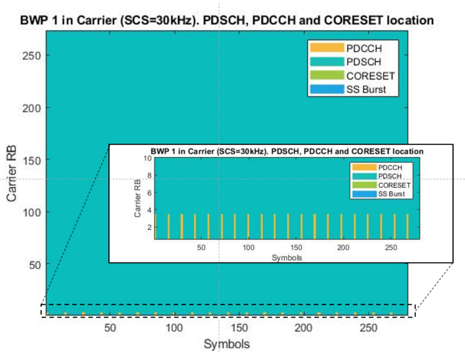
Figure 5. OFDM grid of NR-FR1-TM3.1a waveform with 100 MHz bandwidth and 30 kHz subcarrier spacing with a detail of the lower 10 resource blocks.
