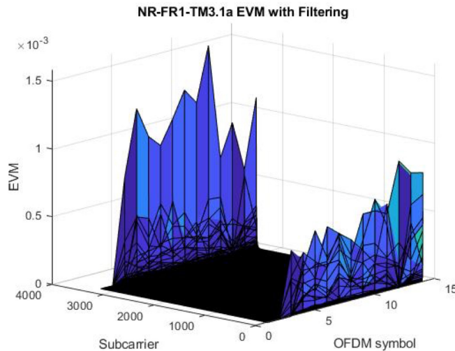
Figure 9. EVM of the filtered NR-FR1-TM3.1a waveform for each resource element in the last slot.
