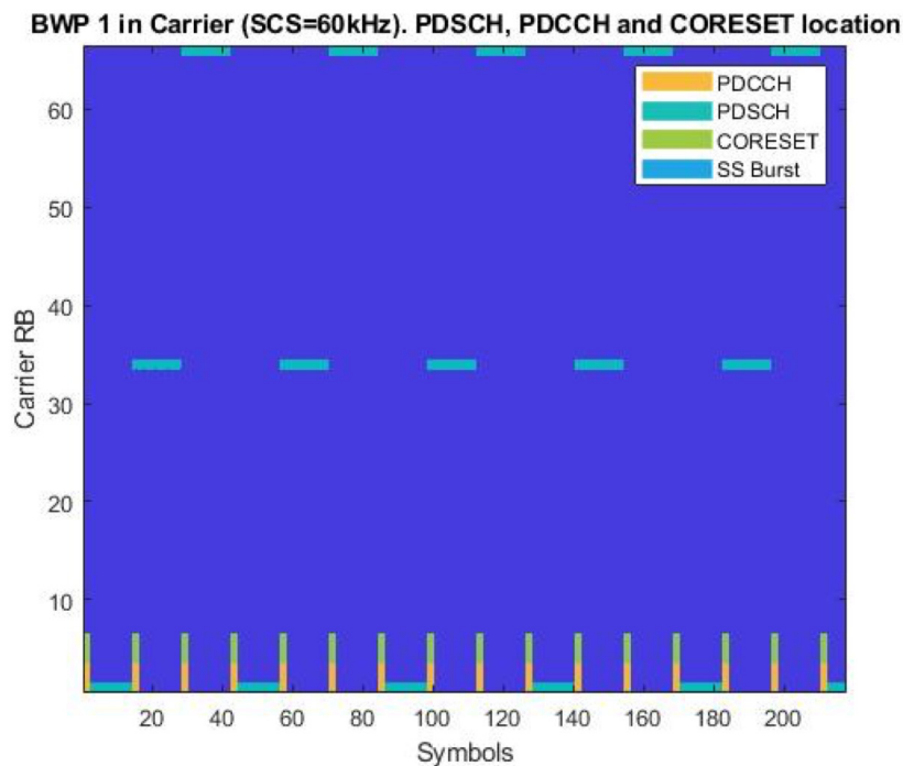
Figure 3. OFDM grid of NR-FR2-TM2 waveform with 50 MHz bandwidth and 60 kHz subcarrier spacing.
