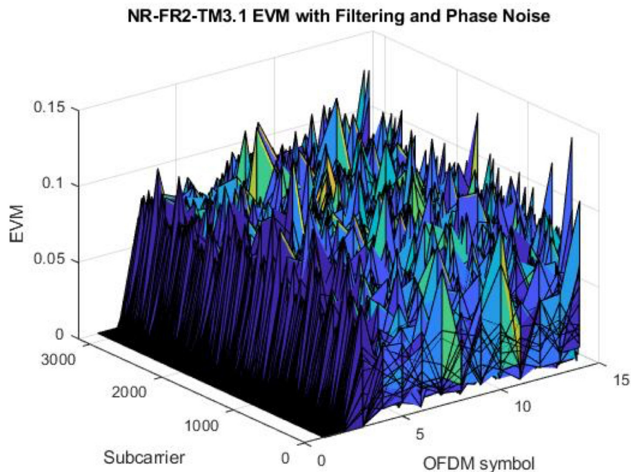
Figure 12. EVM of the NR-FR2-TM3.1 waveform corrupted by phase noise, for each resource element in the last slot.
