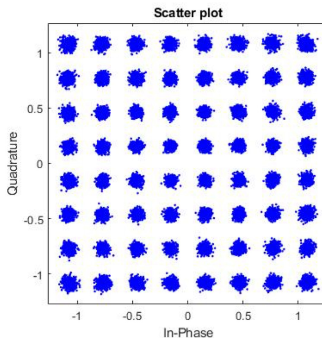
Figure 11. Constellation of NR-FR2-TM3.1 waveform corrupted by phase noise.
