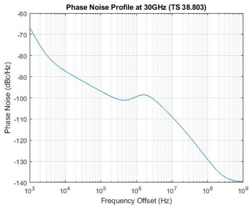
Figure 10. Model of phase noise according to 30 GHz example in 3GPP TS 38.803.
