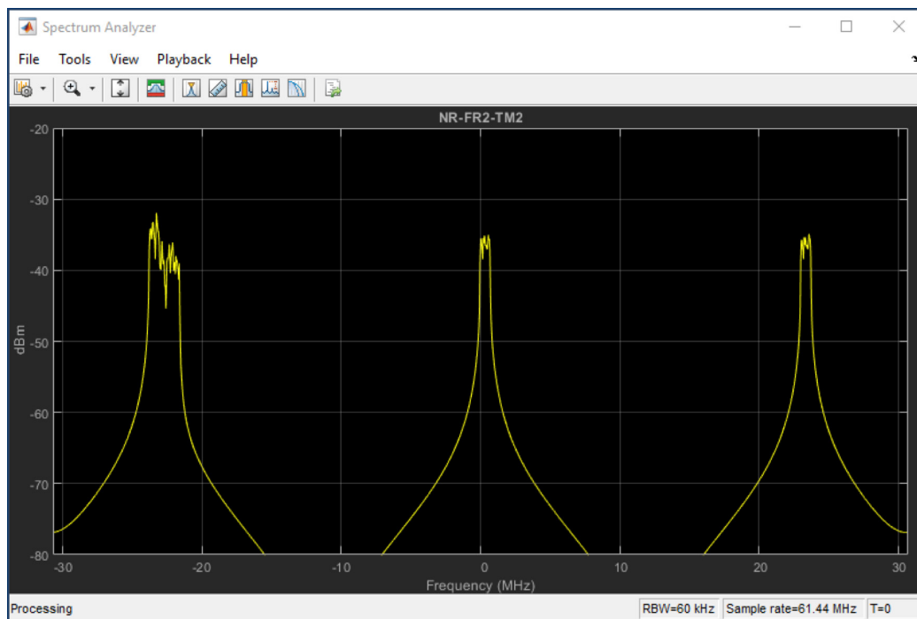
Figure 2. Spectrum of NR-FR2-TM2 waveform with 50 MHz bandwidth and 60 kHz subcarrier spacing.
