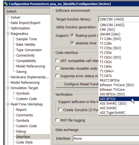
Figure 7 Selecting the TFL for Blackfin 53x
